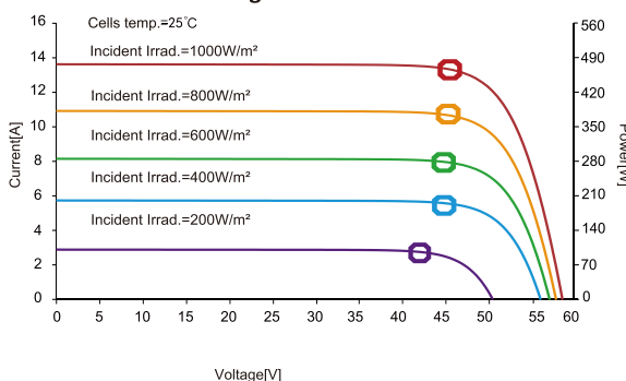
Current-Voltage Curve
