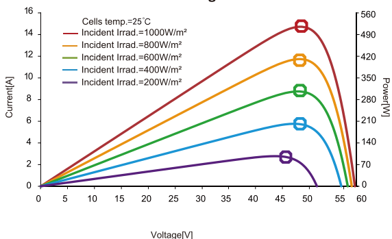
Power-Voltage Curve
